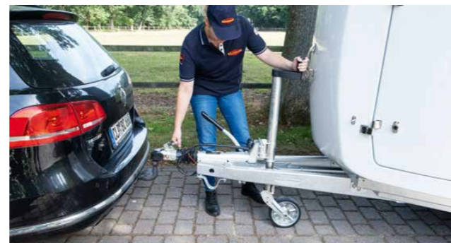
Easy manoeuvring due to the automatic jockey wheel – extra-long with an easy-to-handle crank and optimally positioned manoeuvring handle, perfect to use, even in cold weather.
