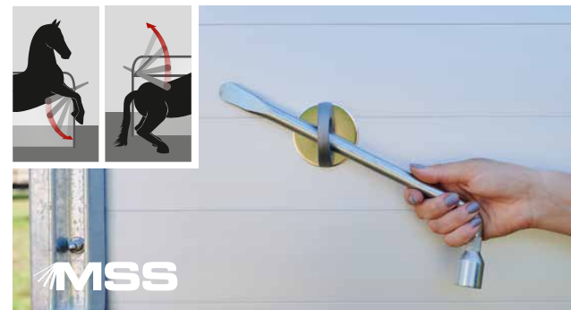
Fast safety in emergencies with the track-proven Multi Safe safety stall bar panic system (MSS). Can be released at the front and rear. The wheel spanner is included in the standard equipment.
