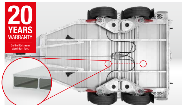
Robust and rot-proof due to the solid quality full aluminium floor with closed profile for reinforcement in the horse compartment.
